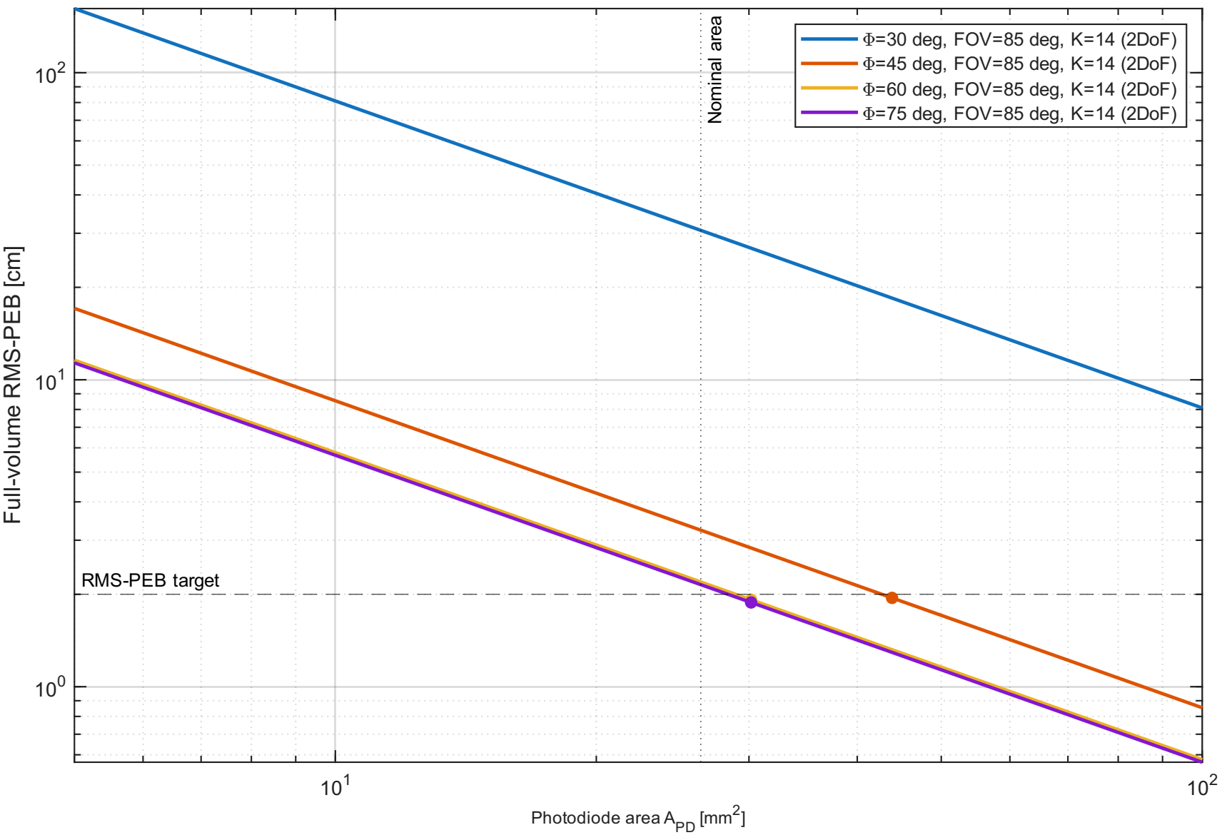
Locally refined 2DoF orientations; constant optical noise PEB scales as 1/A_{PD} : no interior area optimum in this model
